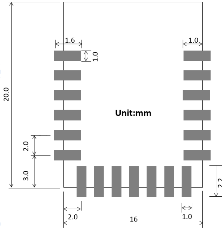
Fig. 3.3 PCB Layout for ESPC3-05
