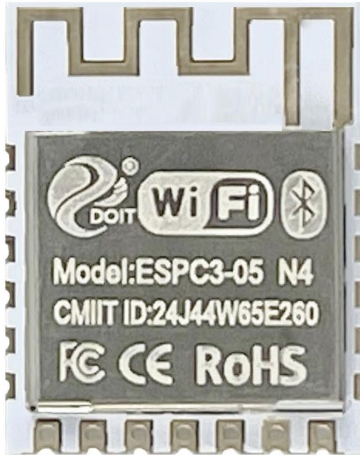
Fig.3.1 Shape for ESPC3-05
