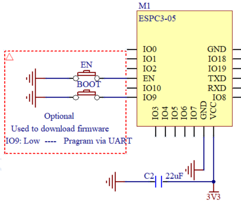
Fig.9.1 Minimum System
