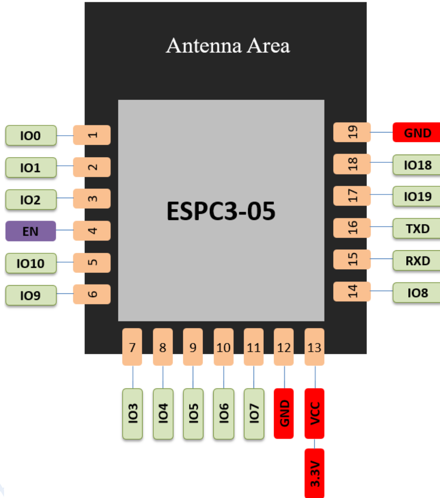
Fig.2.1 ESPC3-05 Pins Definition
