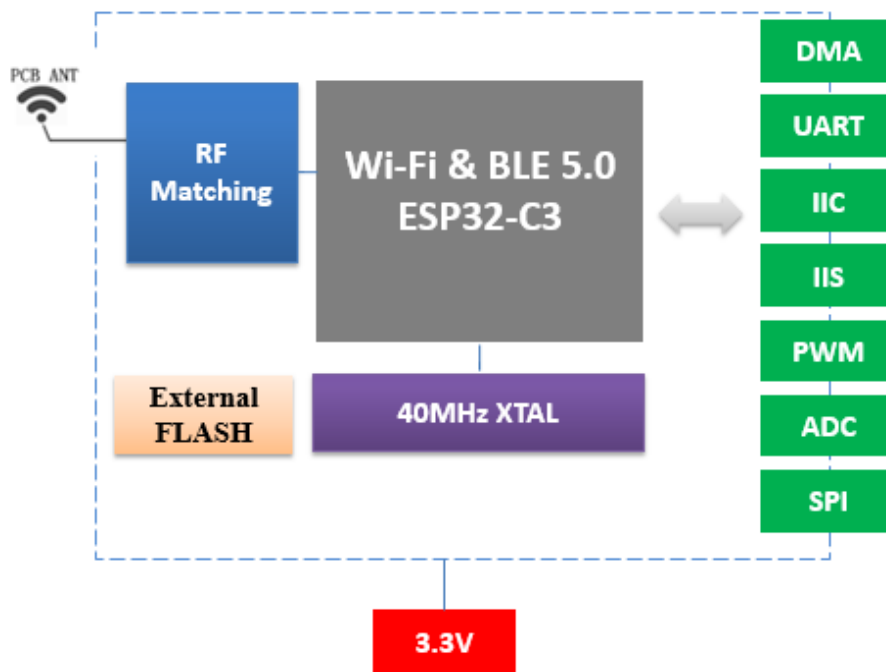
Fig.1.1 ESPC3-05 Module Structure
