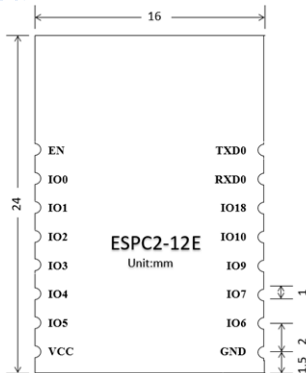
Shape of ESPC2-12E
