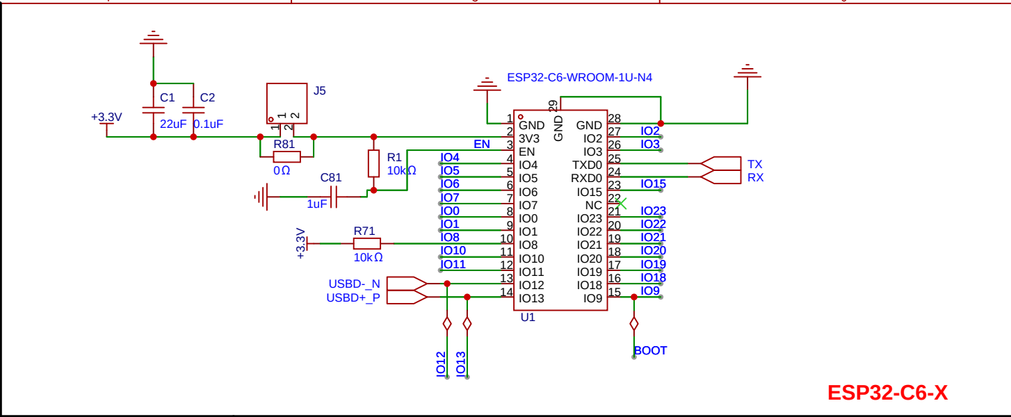
UART-light
